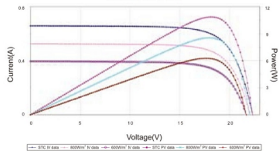
Module IV Graph 10W
