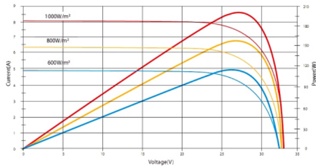
Mono-crystalline Modules 210W
